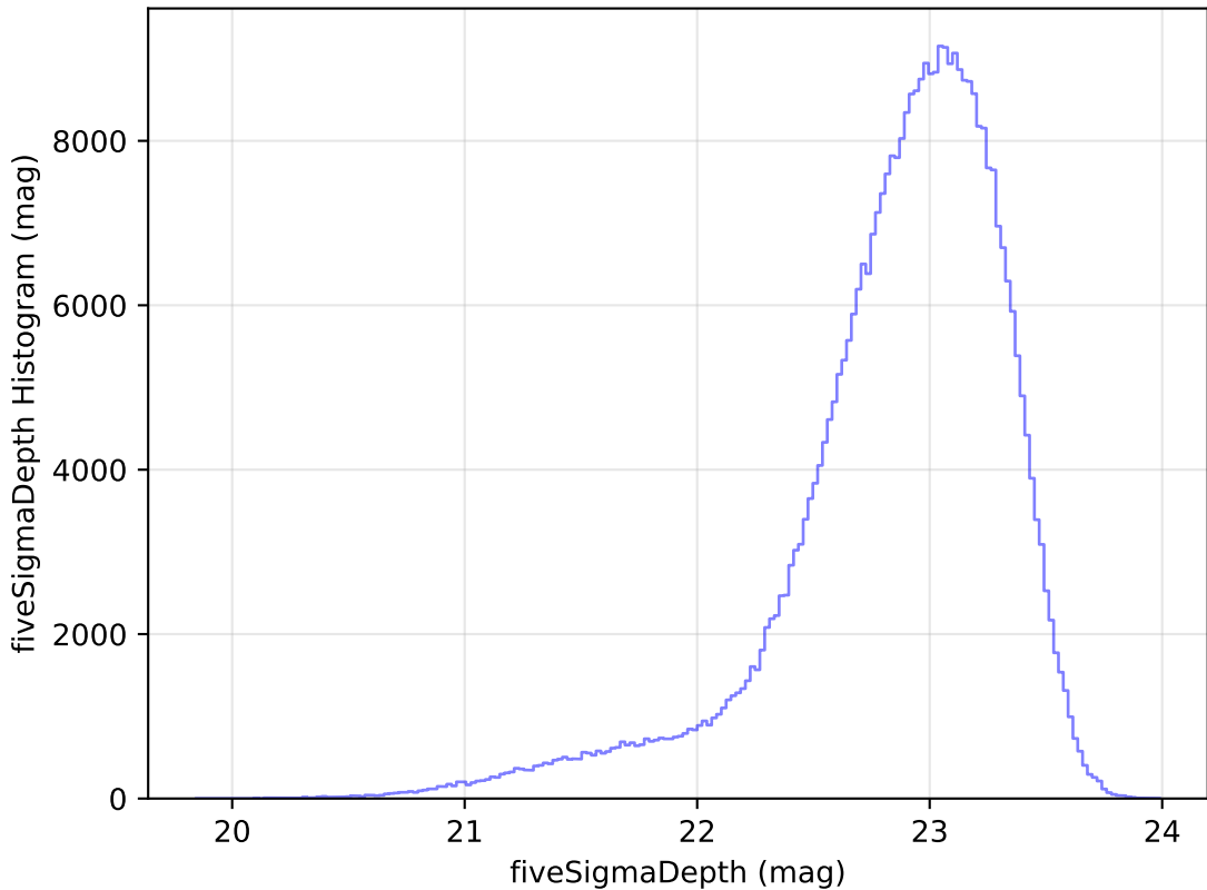
internal_u_expt60_nscale1.2v3.4_10yrs z: fiveSigmaDepth Histogram
