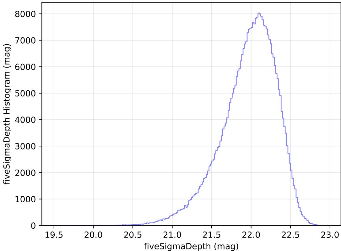
internal_u_expt60_nscale1.2v3.4_10yrs y: fiveSigmaDepth Histogram
