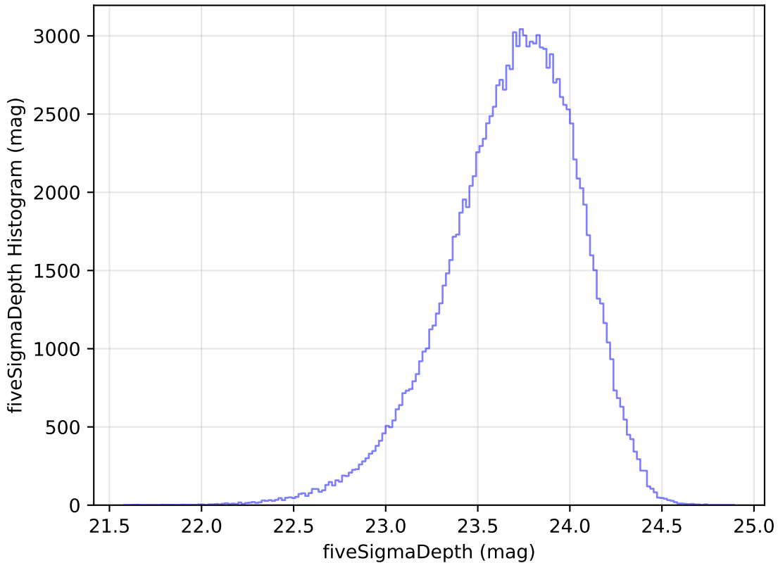
internal_u_expt60_nscale1.2v3.4_10yrs u: fiveSigmaDepth Histogram
