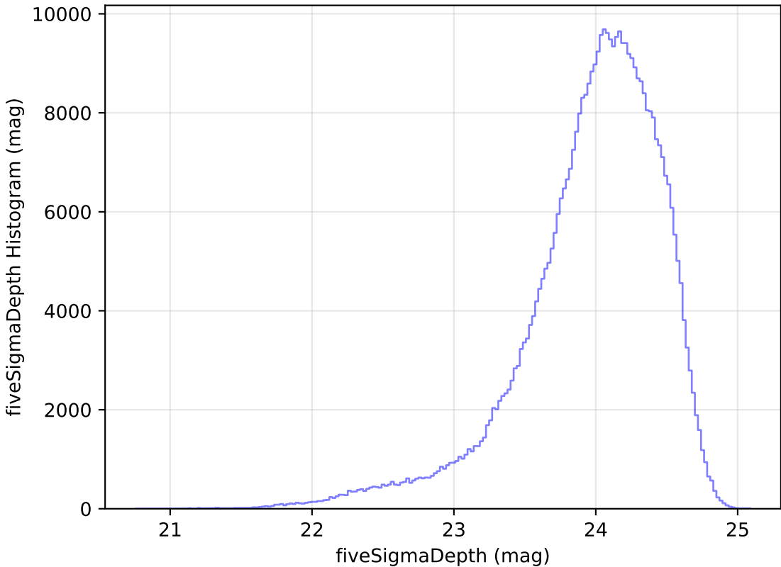
internal_u_expt60_nscale1.2v3.4_10yrs r: fiveSigmaDepth Histogram
