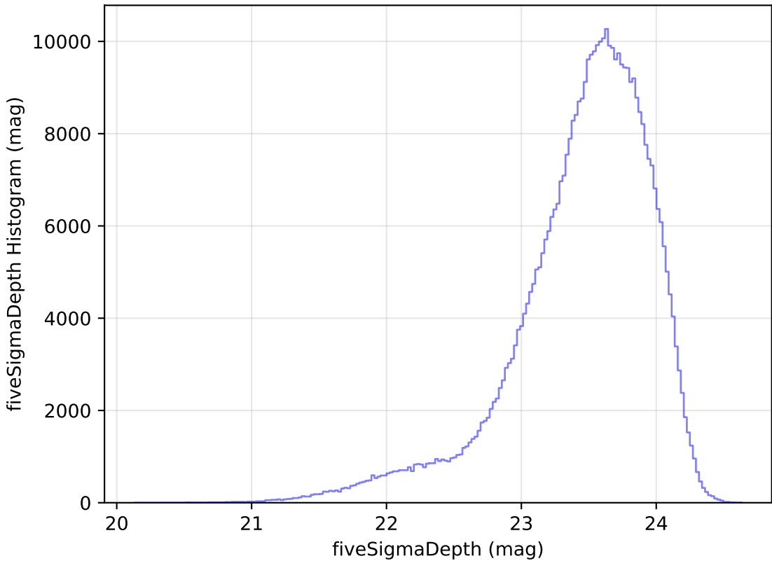
internal_u_expt60_nscale1.2v3.4_10yrs i: fiveSigmaDepth Histogram
