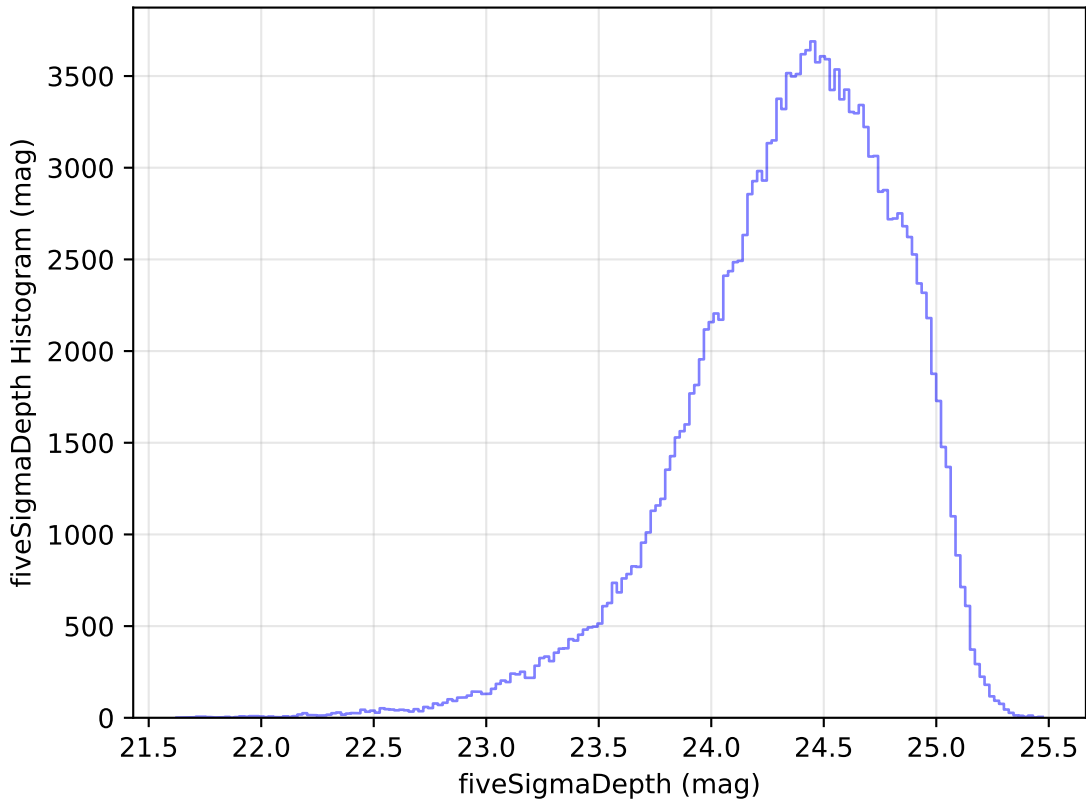
internal_u_expt60_nscale1.2v3.4_10yrs g: fiveSigmaDepth Histogram
