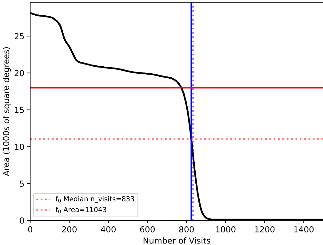
internal_u_expt60_nscale1.2v3.4_10yrs : fO
