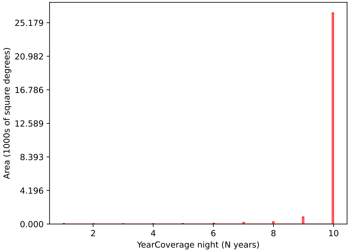
internal_u_expt60_nscale1.2v3.4_10yrs i band: YearCoverage night
