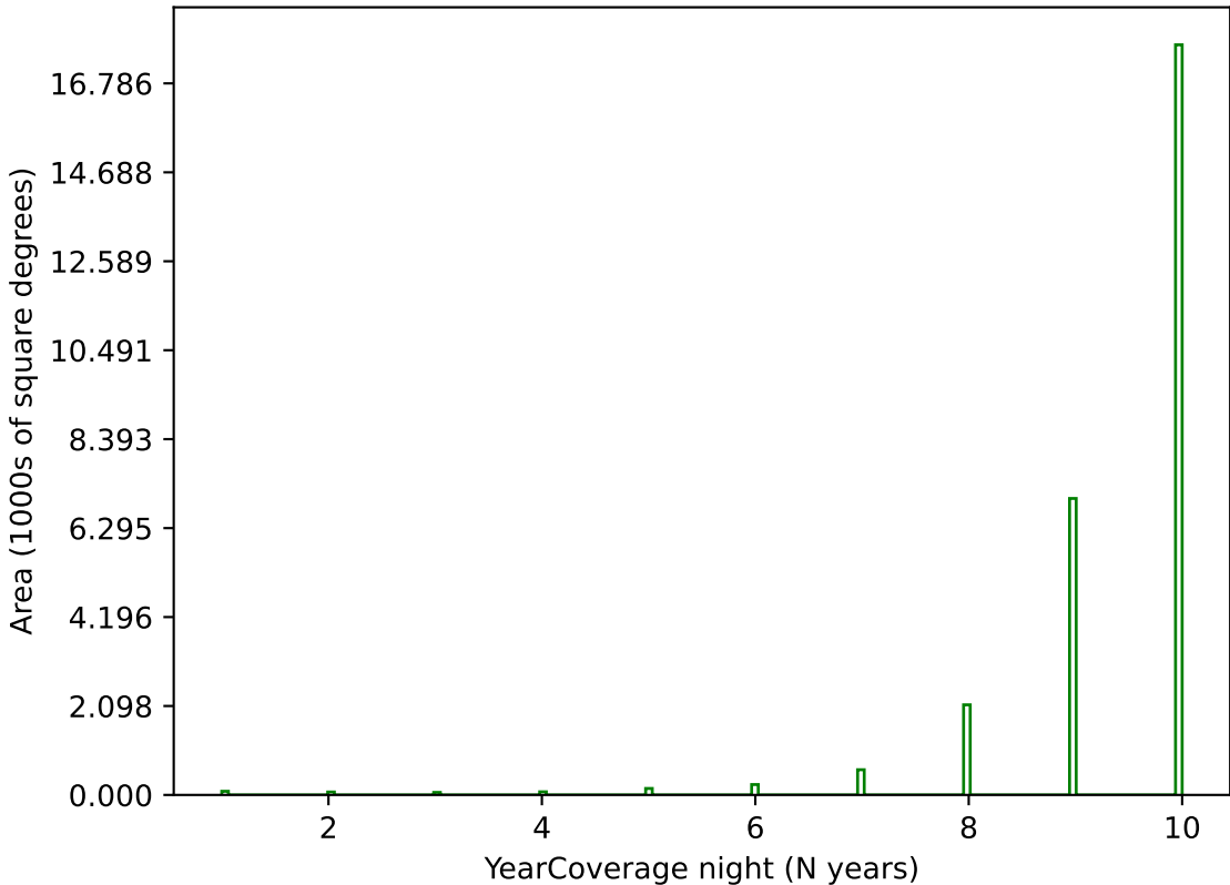
internal_u_expt60_nscale1.2v3.4_10yrs g band: YearCoverage night
