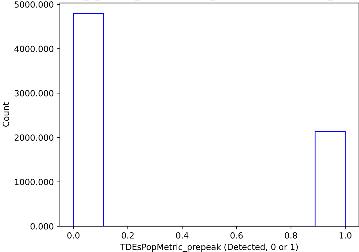
internal_u_expt60_nscale1.2v3.4_10yrs : TDEsPopMetric_prepeak
