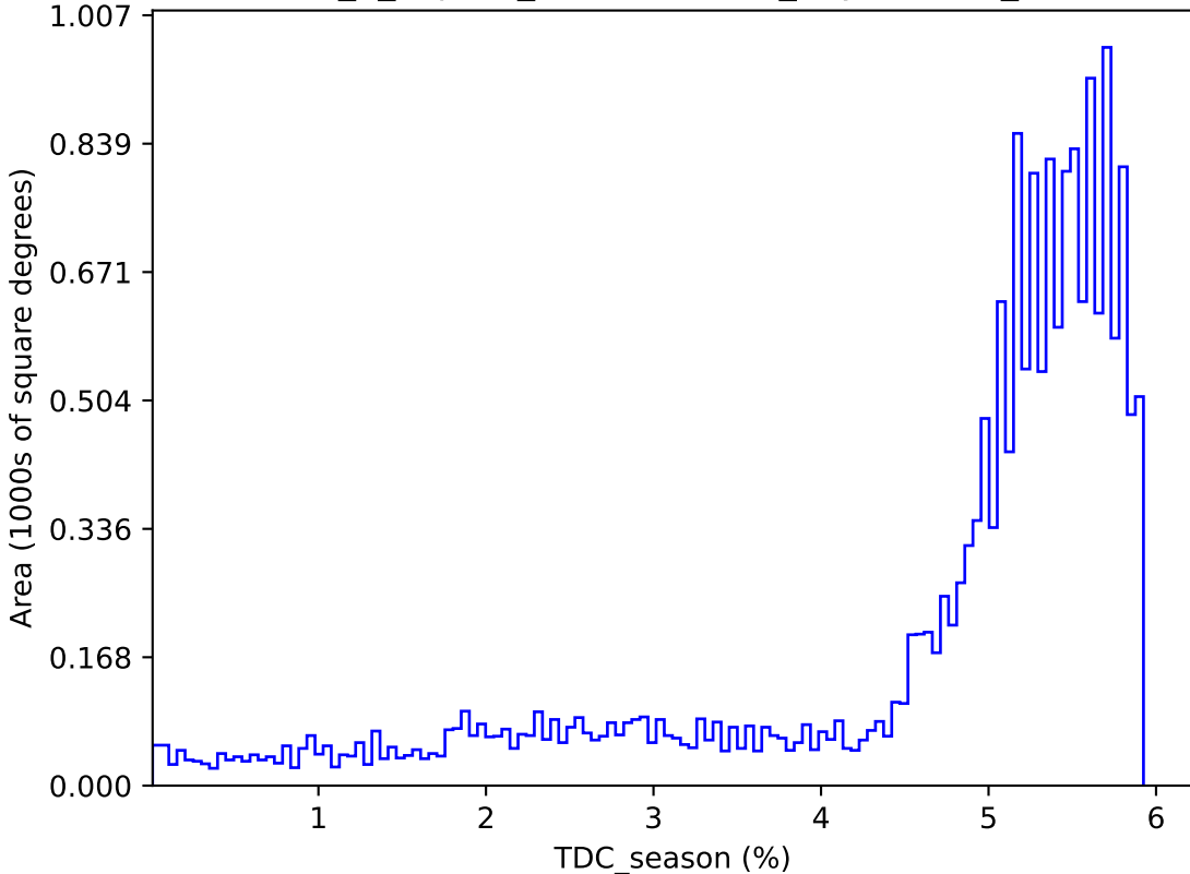
internal_u_expt60_nscale1.2v3.4_10yrs : TDC_season
