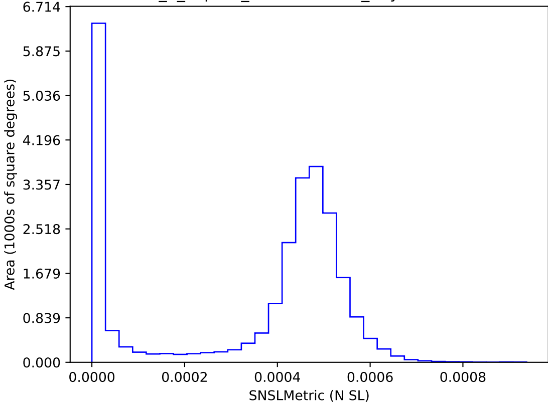
internal_u_expt60_nscale1.2v3.4_10yrs : SNSLMetric
