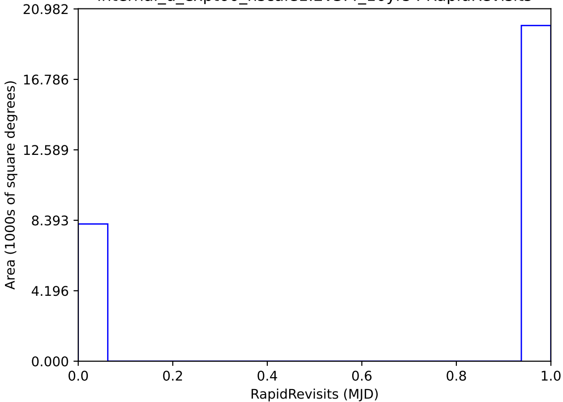
internal_u_expt60_nscale1.2v3.4_10yrs : RapidRevisits
