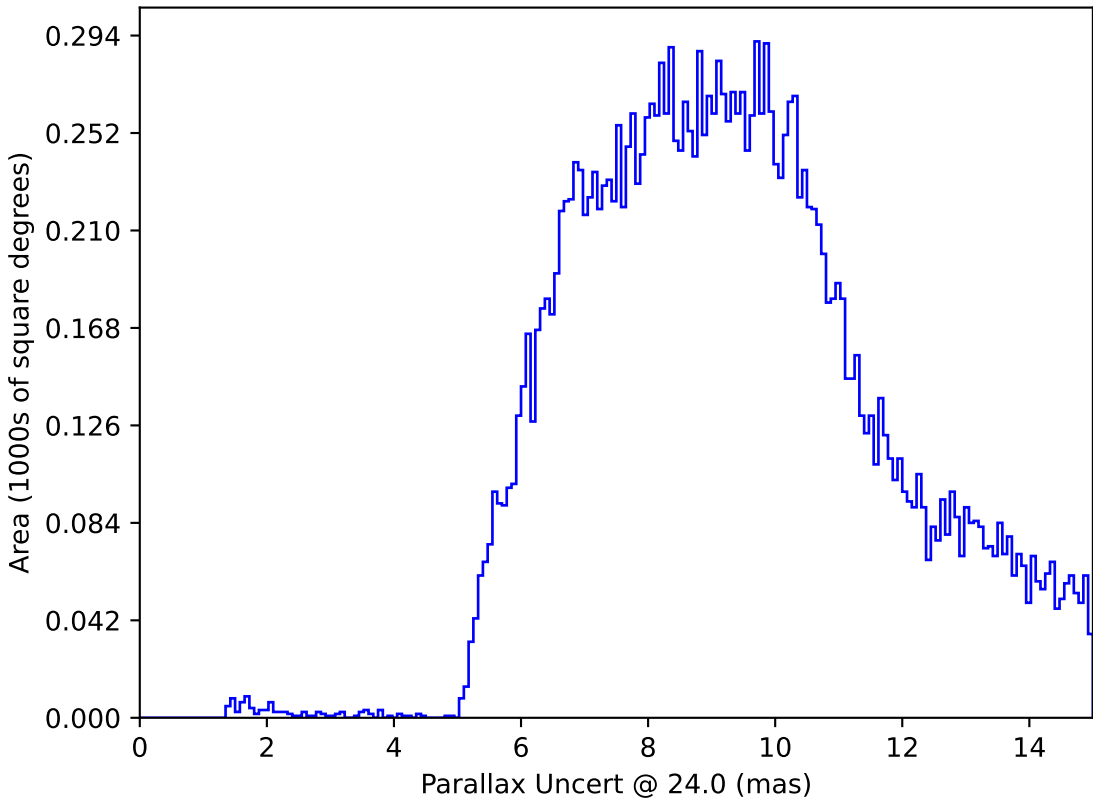
internal_u_expt60_nscale1.2v3.4_10yrs : Parallax Uncert @ 24.0
