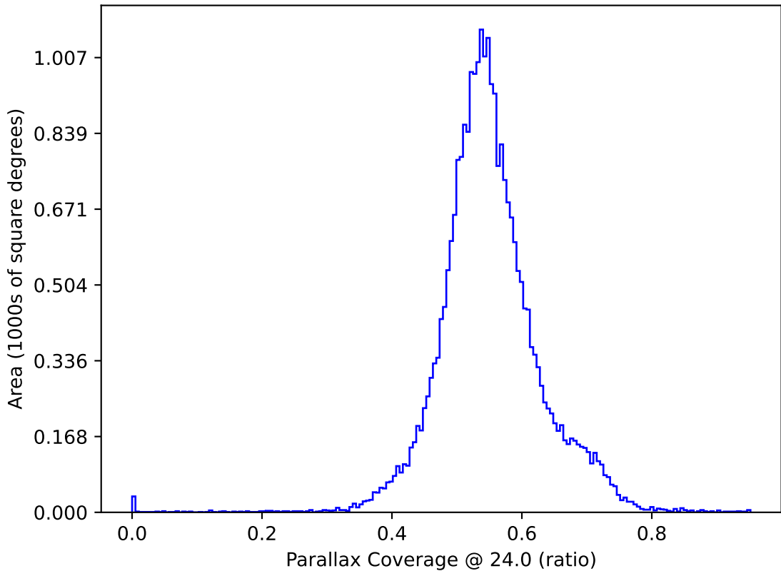
internal_u_expt60_nscale1.2v3.4_10yrs : Parallax Coverage @ 24.0
