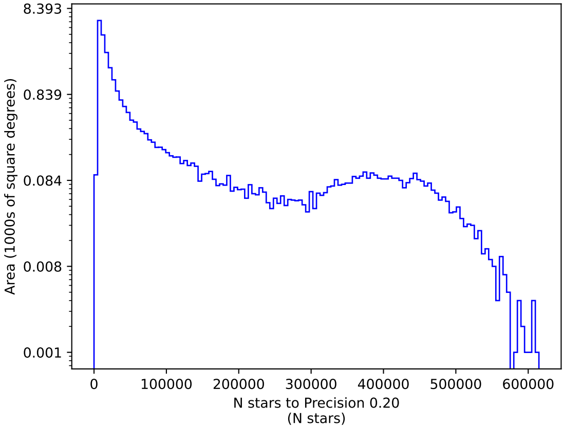
internal_u_expt60_nscale1.2v3.4_10yrs z: N stars to Precision 0.20
