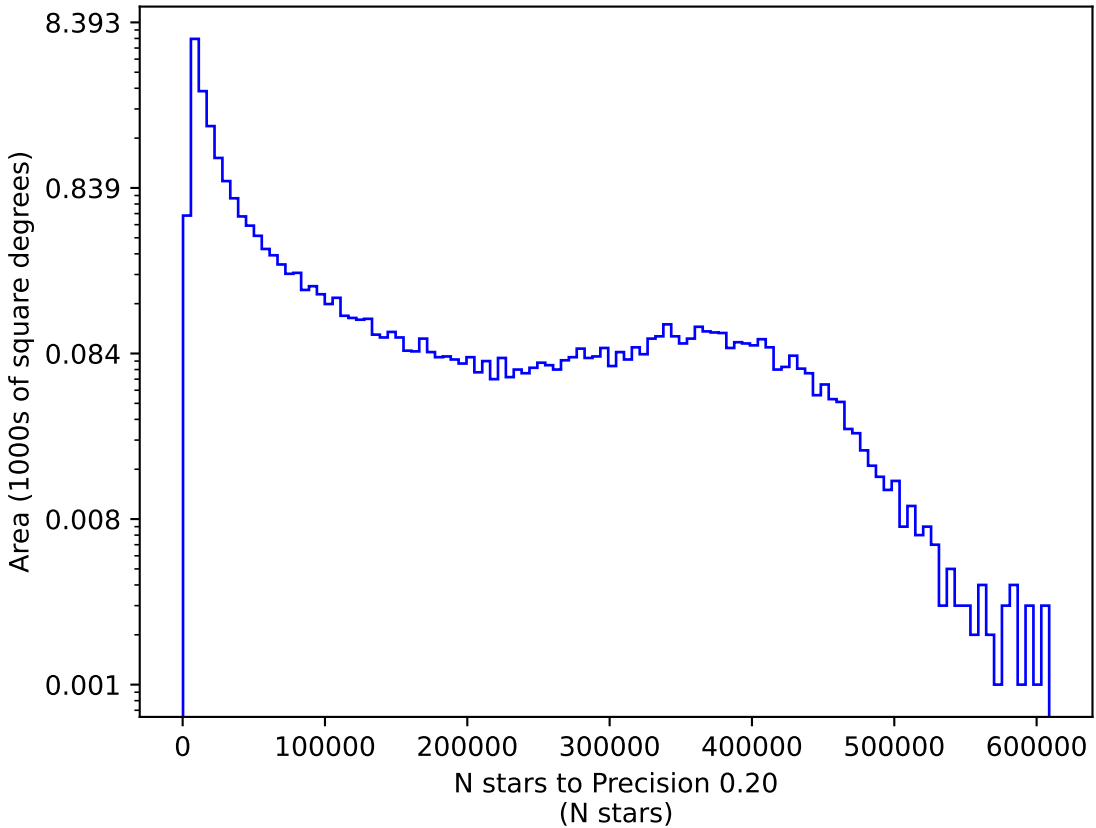
internal_u_expt60_nscale1.2v3.4_10yrs y: N stars to Precision 0.20
