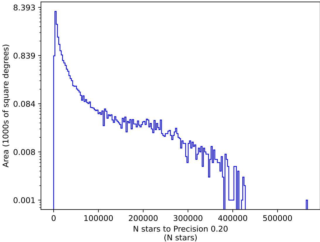
internal_u_expt60_nscale1.2v3.4_10yrs u: N stars to Precision 0.20
