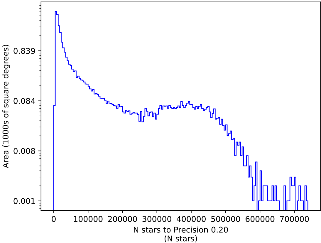
internal_u_expt60_nscale1.2v3.4_10yrs r: N stars to Precision 0.20
