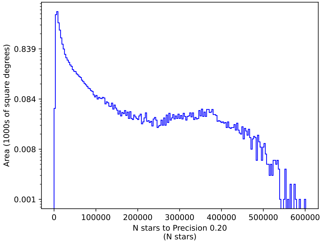
internal_u_expt60_nscale1.2v3.4_10yrs g: N stars to Precision 0.20
