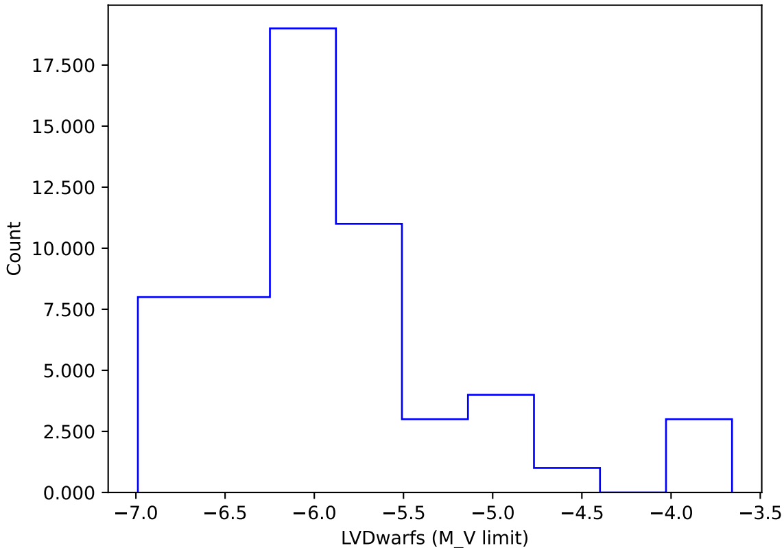
internal_u_expt60_nscale1.2v3.4_10yrs gi: LVDwarfs
