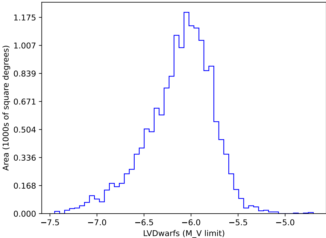
internal_u_expt60_nscale1.2v3.4_10yrs gi: LVDwarfs
