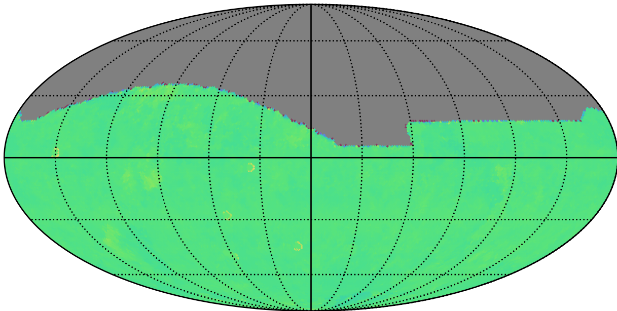
internal_u_expt60_nscale1.2v3.4_10yrs i: Kuiper rotTelPos
