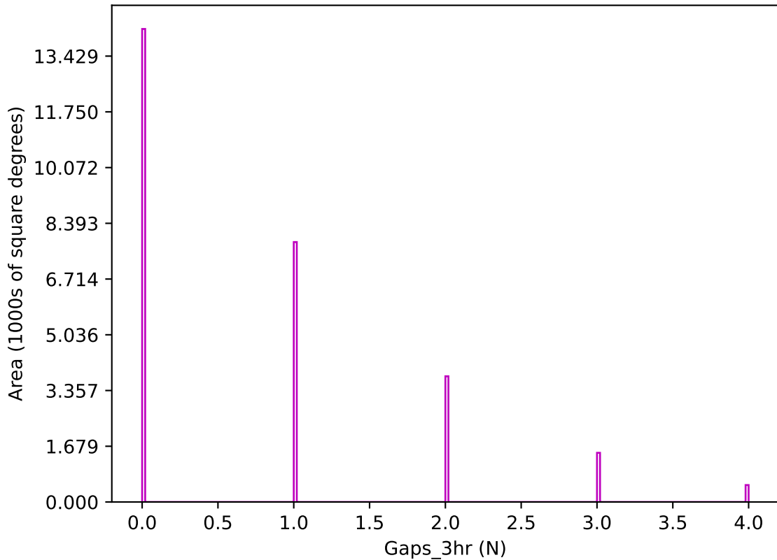
internal_u_expt60_nscale1.2v3.4_10yrs z band: Gaps_3hr
