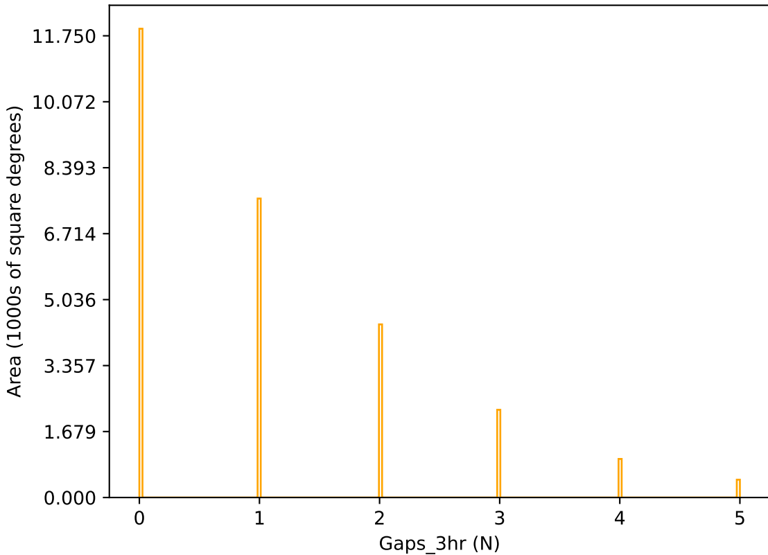
internal_u_expt60_nscale1.2v3.4_10yrs r band: Gaps_3hr
