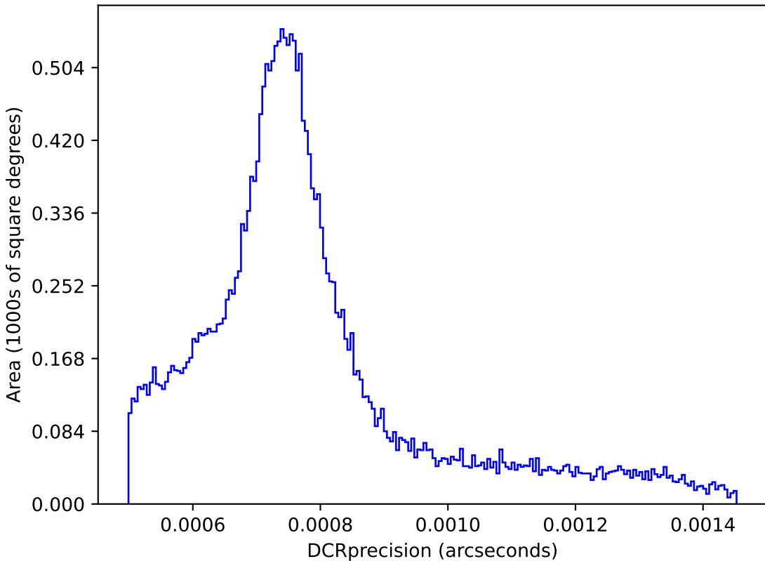
internal_u_expt60_nscale1.2v3.4_10yrs : DCRprecision
