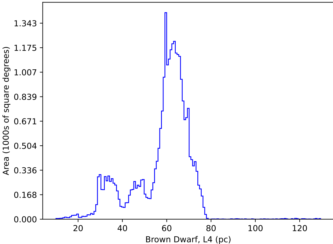
internal_u_expt60_nscale1.2v3.4_10yrs : Brown Dwarf, L4
