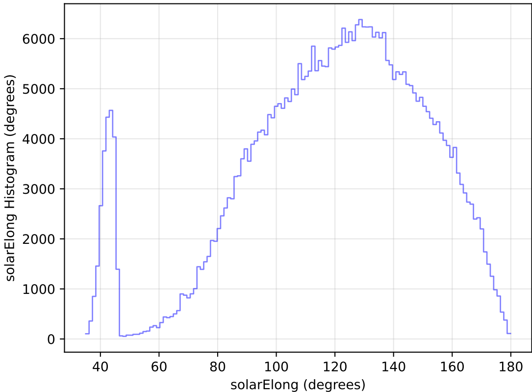
internal_u_expt60_nscale1.2v3.4_10yrs WFD z band: solarElong Histogram
