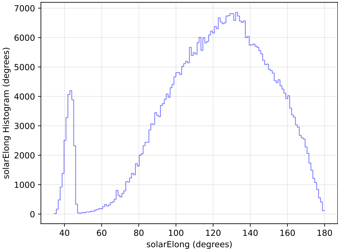
internal_u_expt60_nscale1.2v3.4_10yrs WFD i band: solarElong Histogram
