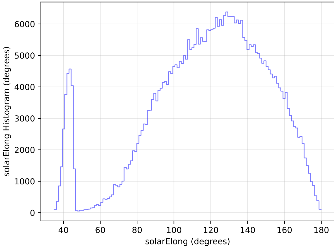
internal_u_expt60_nscale1.2v3.4_10yrs All sky z band: solarElong Histogram
