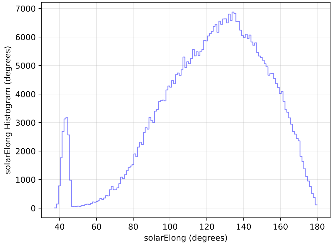
internal_u_expt60_nscale1.2v3.4_10yrs All sky r band: solarElong Histogram
