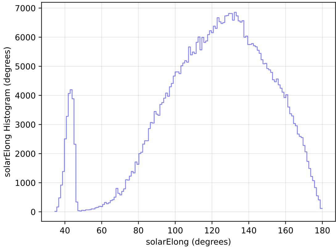
internal_u_expt60_nscale1.2v3.4_10yrs All sky i band: solarElong Histogram
