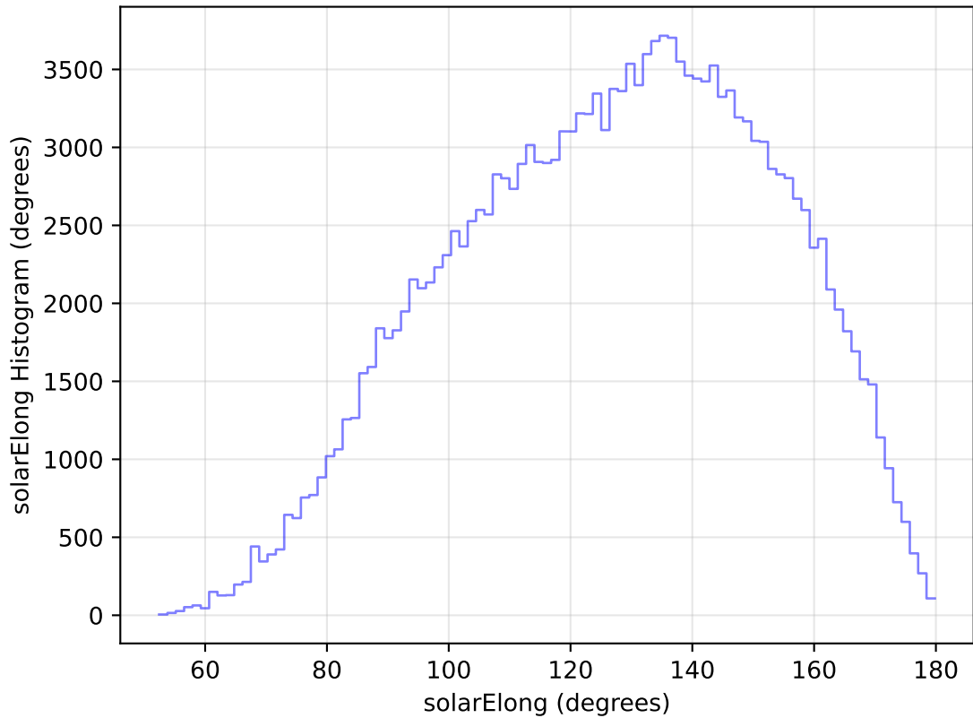
internal_u_expt60_nscale1.2v3.4_10yrs All sky g band: solarElong Histogram
