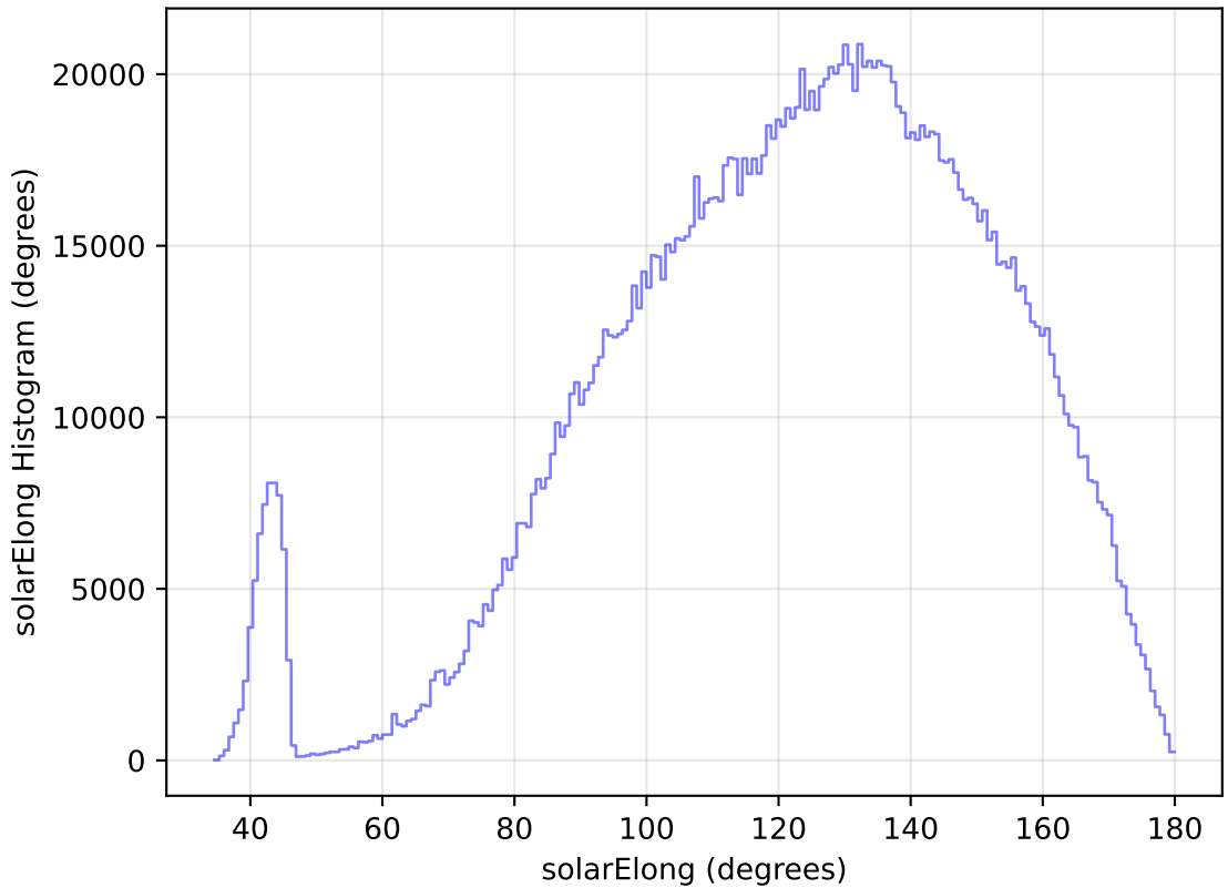
internal_u_expt60_nscale1.2v3.4_10yrs All sky all bands: solarElong Histogram
