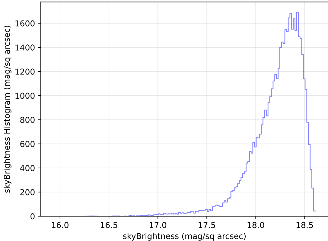
internal_u_expt60_nscale1.2v3.4_10yrs Yr 1 y band: skyBrightness Histogram
