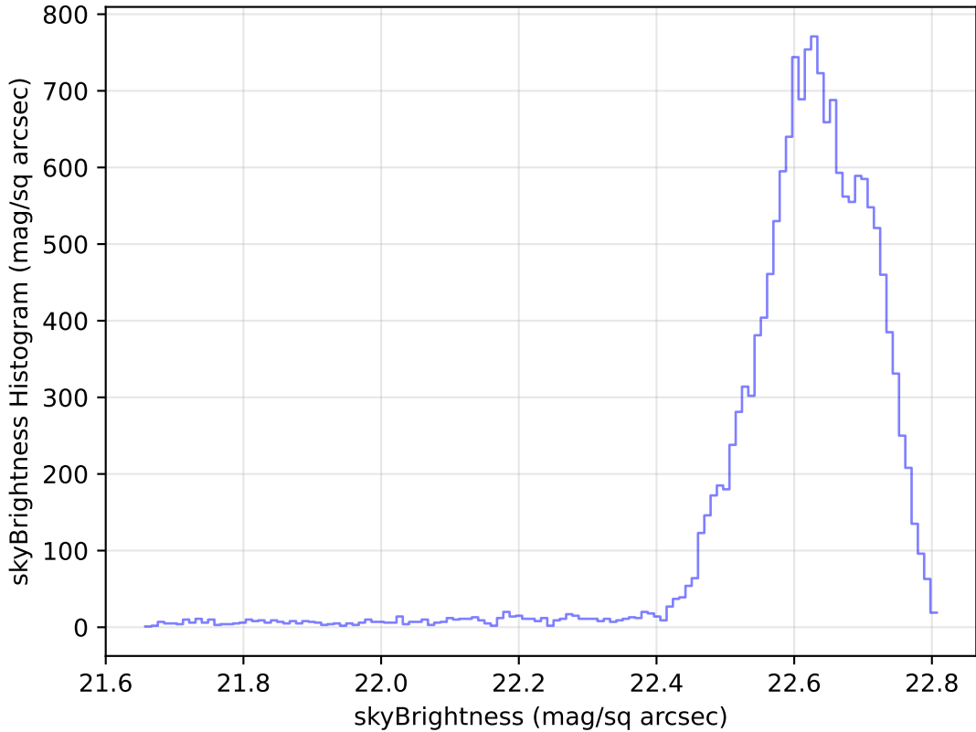
internal_u_expt60_nscale1.2v3.4_10yrs Yr 1 u band: skyBrightness Histogram
