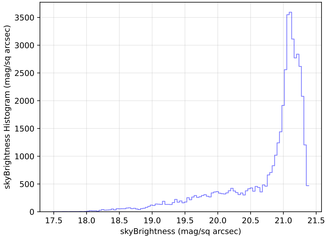
internal_u_expt60_nscale1.2v3.4_10yrs Yr 1 r band: skyBrightness Histogram
