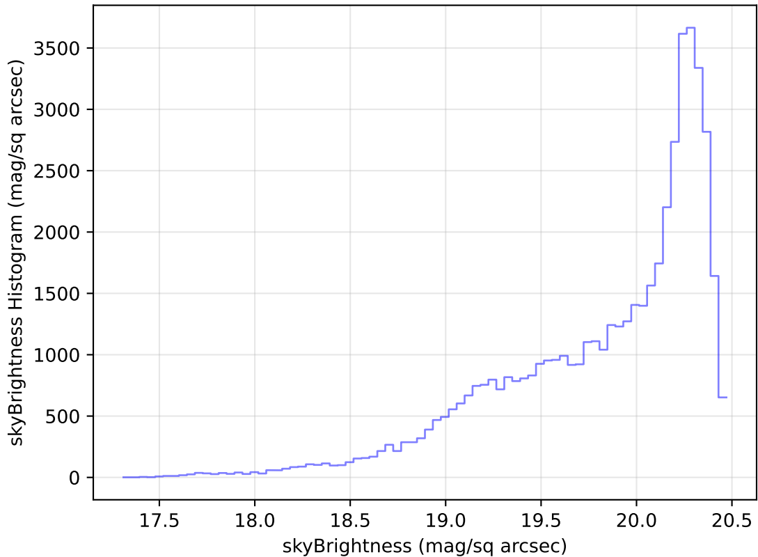
internal_u_expt60_nscale1.2v3.4_10yrs Yr 1 i band: skyBrightness Histogram
