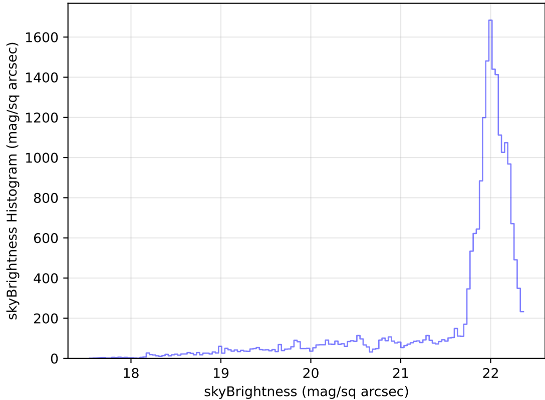
internal_u_expt60_nscale1.2v3.4_10yrs Yr 1 g band: skyBrightness Histogram
