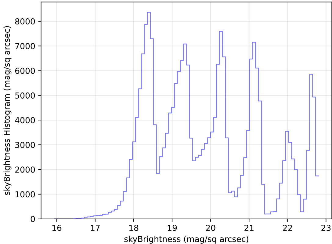
internal_u_expt60_nscale1.2v3.4_10yrs Yr 1 all bands: skyBrightness Histogram
