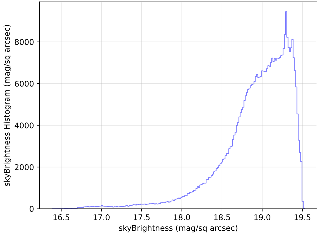
internal_u_expt60_nscale1.2v3.4_10yrs WFD z band: skyBrightness Histogram
