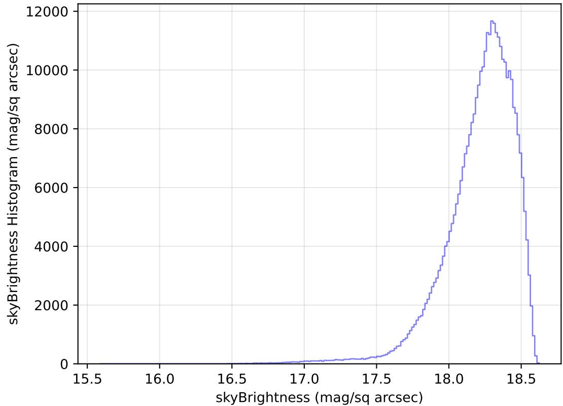
internal_u_expt60_nscale1.2v3.4_10yrs WFD y band: skyBrightness Histogram
