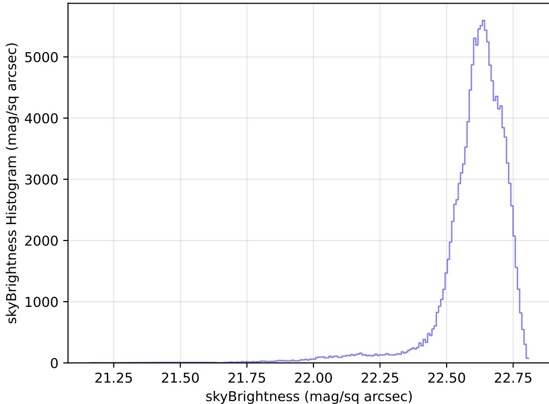
internal_u_expt60_nscale1.2v3.4_10yrs WFD u band: skyBrightness Histogram
