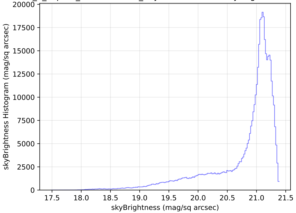
internal_u_expt60_nscale1.2v3.4_10yrs WFD r band: skyBrightness Histogram
