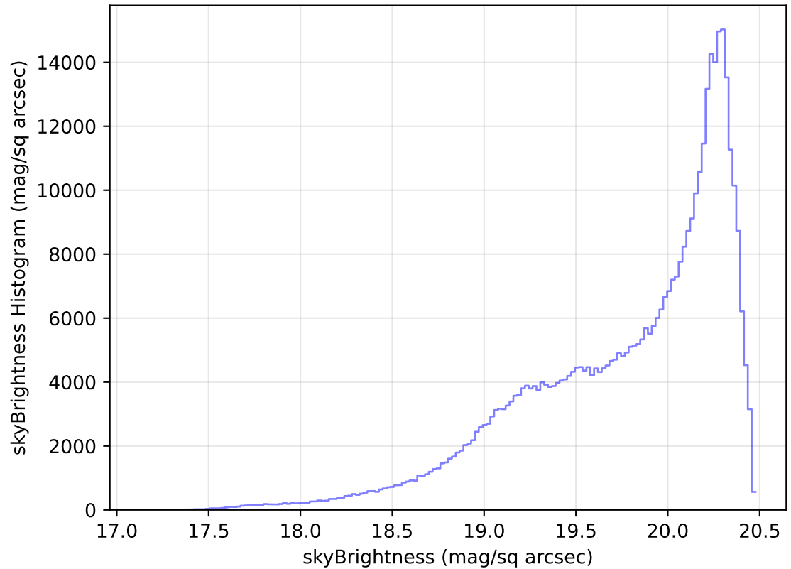
internal_u_expt60_nscale1.2v3.4_10yrs WFD i band: skyBrightness Histogram
