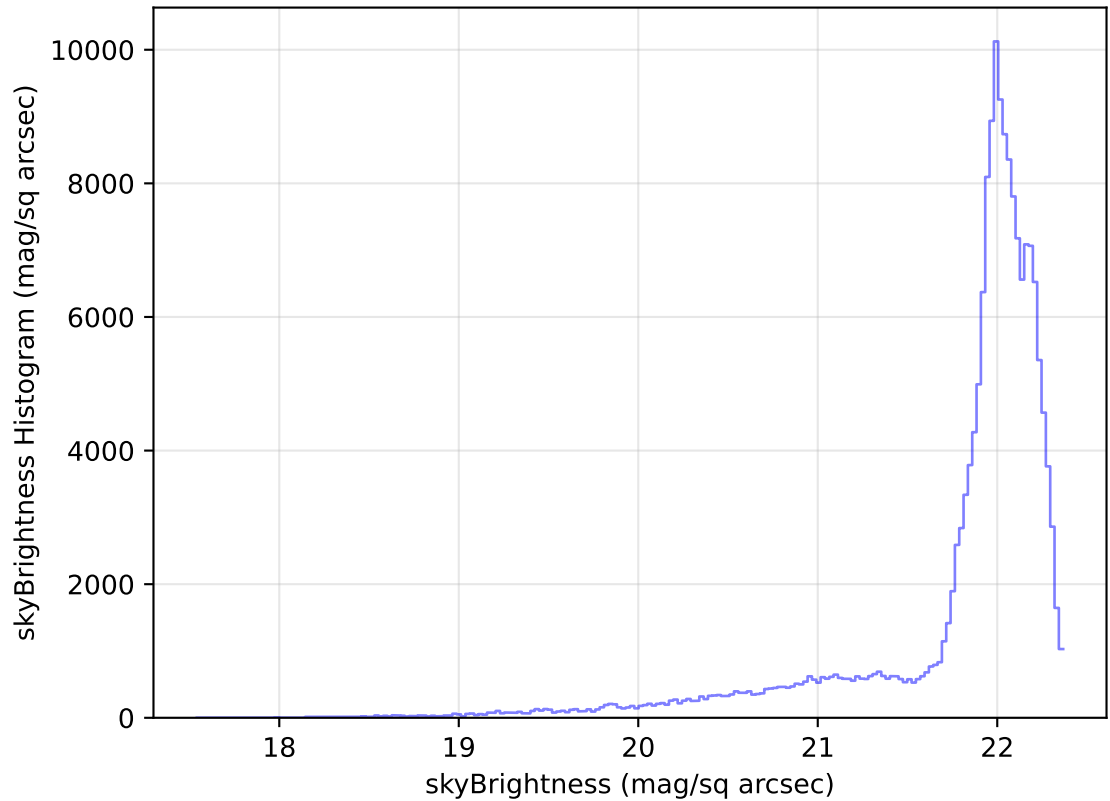
internal_u_expt60_nscale1.2v3.4_10yrs WFD g band: skyBrightness Histogram
