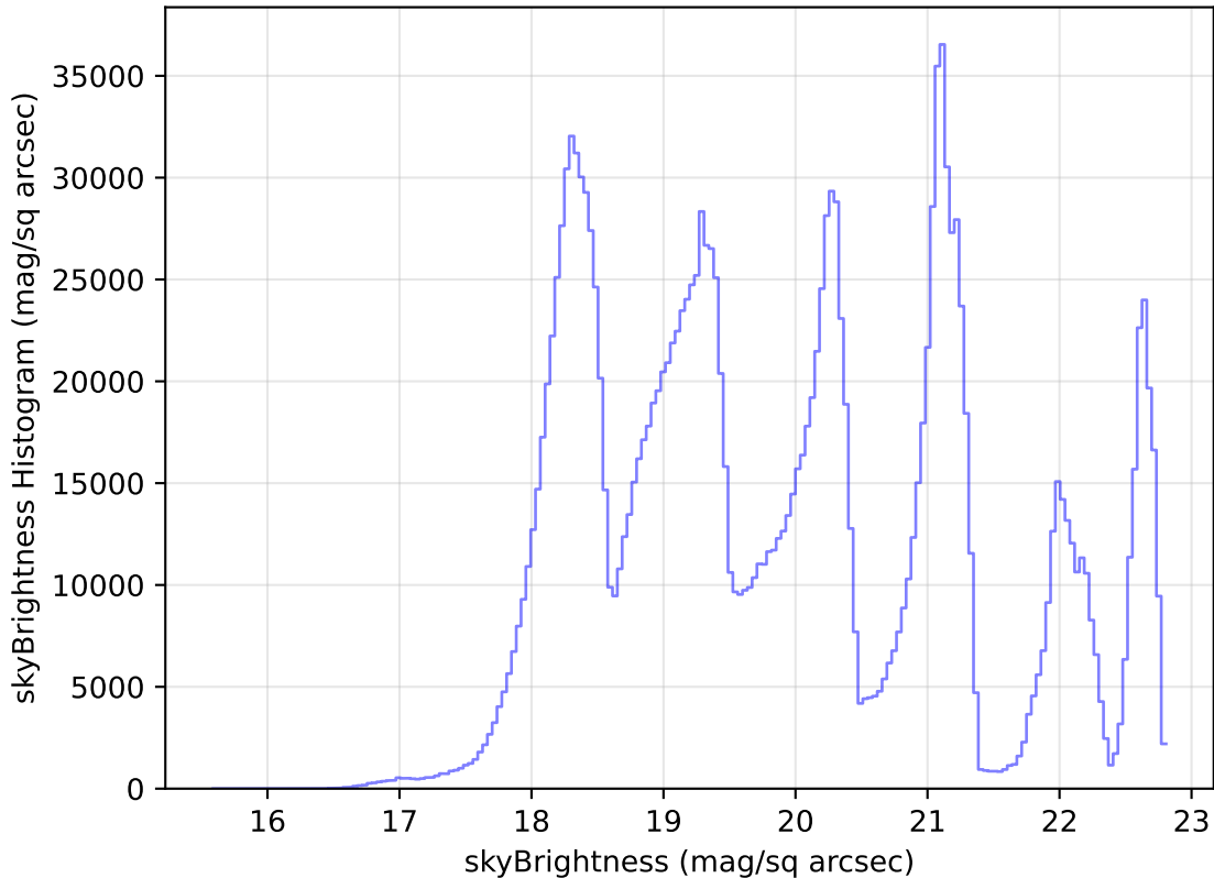
internal_u_expt60_nscale1.2v3.4_10yrs WFD all bands: skyBrightness Histogram
