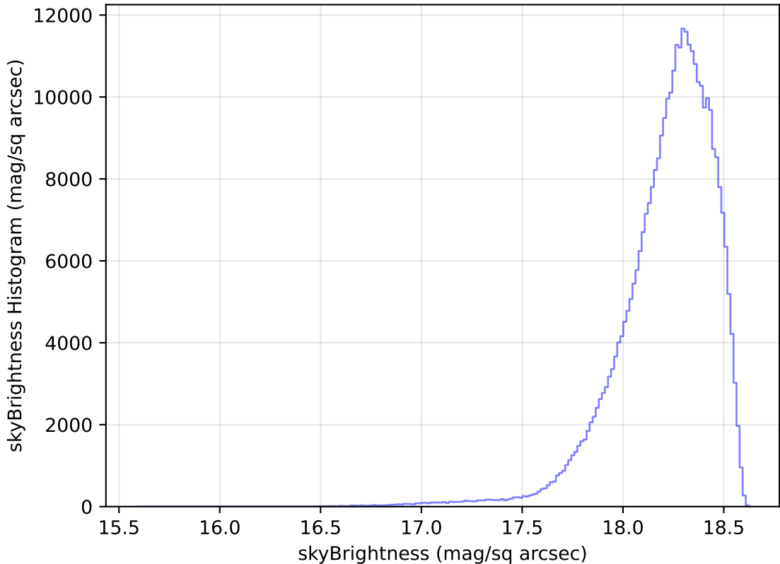
internal_u_expt60_nscale1.2v3.4_10yrs All sky y band: skyBrightness Histogram
