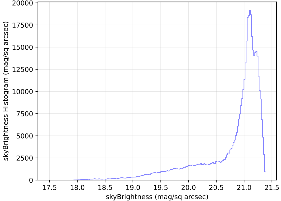
internal_u_expt60_nscale1.2v3.4_10yrs All sky r band: skyBrightness Histogram
