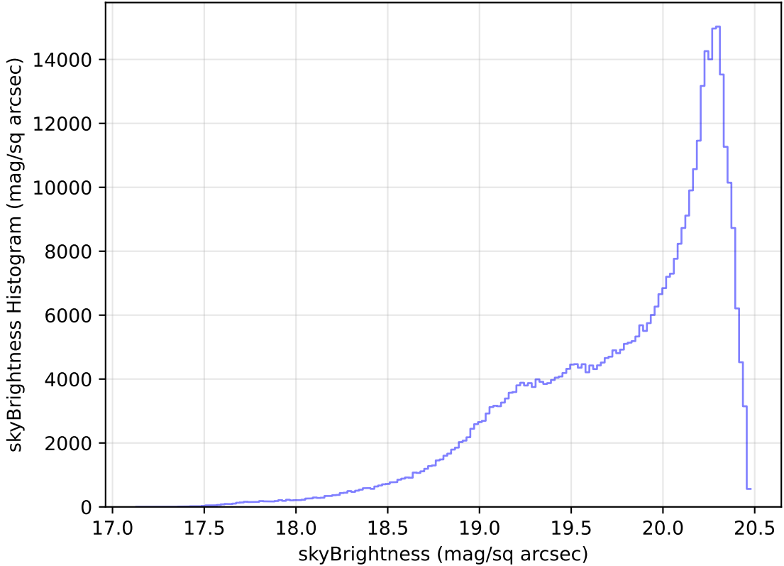
internal_u_expt60_nscale1.2v3.4_10yrs All sky i band: skyBrightness Histogram
